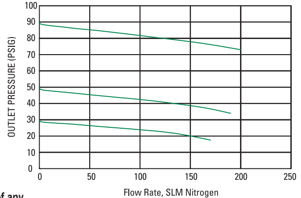
MODEL AZ 1500 HF Flow Curve at 150 psig Inlet Pressure
